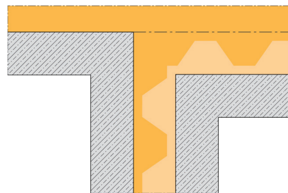
With temporary steel sheet pile retaining walls, the reinforced concrete structure built inside the excavation pit reduces the available surface
